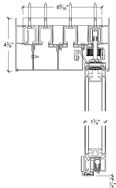
Double glazed in the closed position Verre double en position fermée
