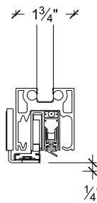
Single glazed in the closed position Verre simple en position fermée
